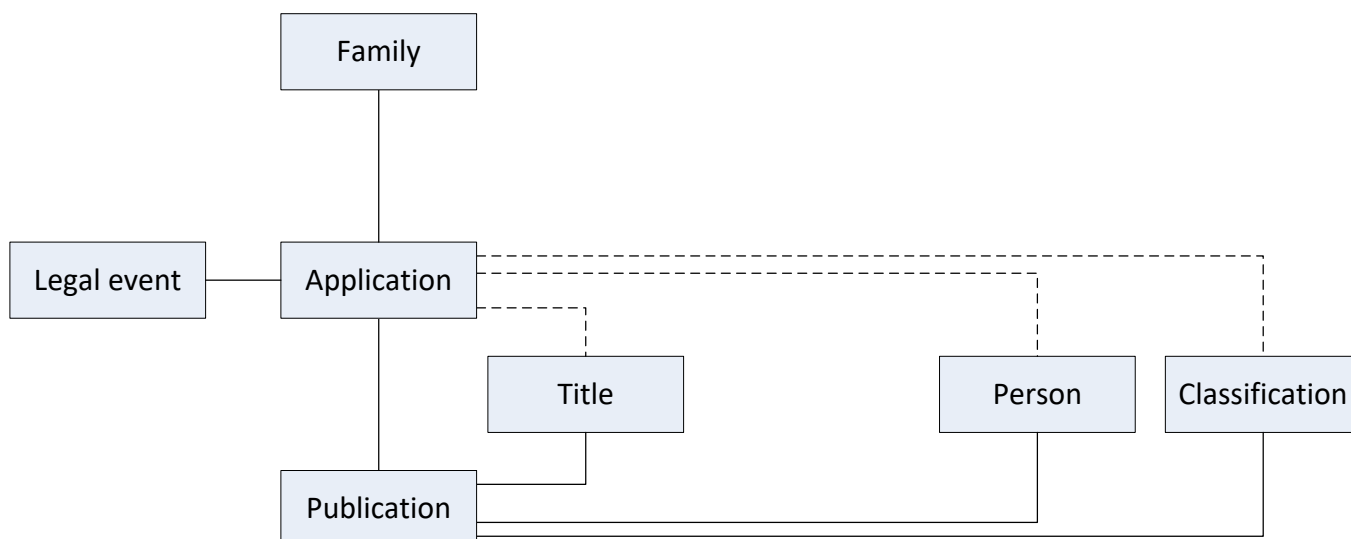
Figure 3: Main Domain Objects in the Family - Application - Publication hierarchy
