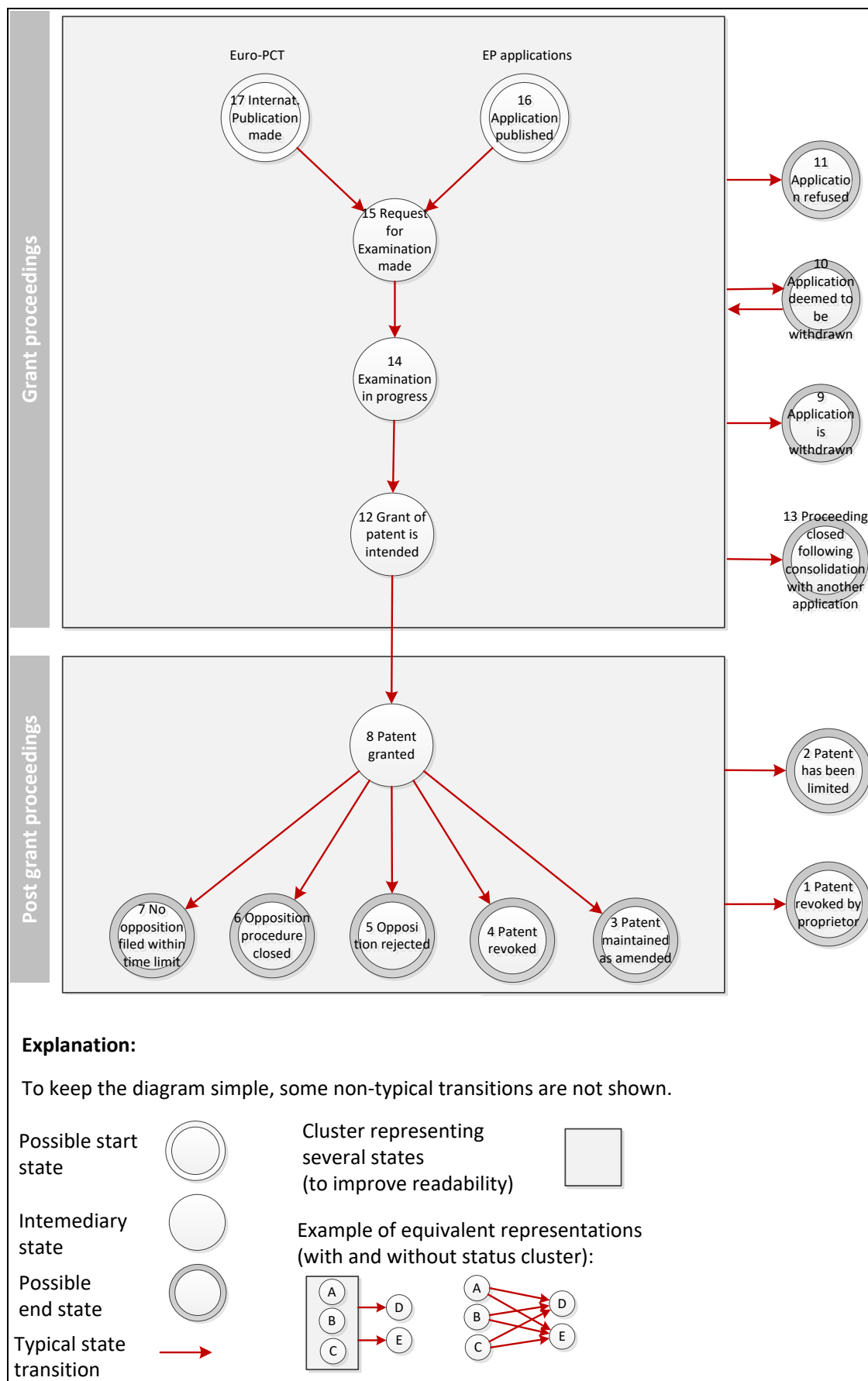
Figure 5: STATUS EP phase: State transition diagram
